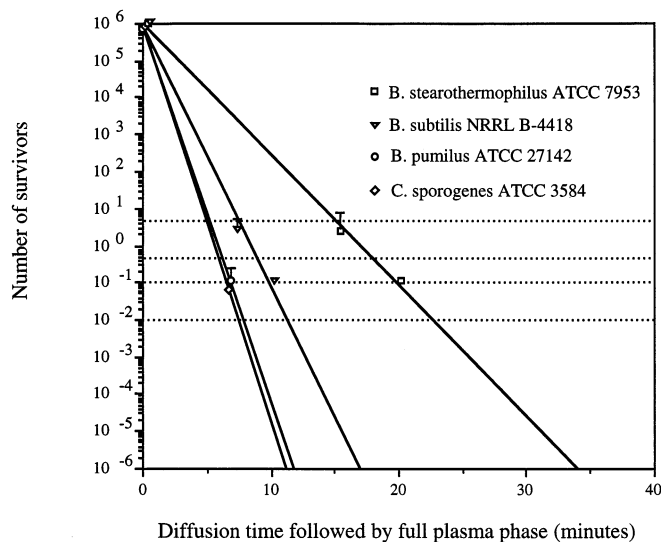
Figure 2. Amount of sterilization time required to achieve organism levels of <10^{-6} for several common, highly resistant bacterial spores ( B. stearothermophilus , B. subtilis , B. pumilus and C. sporogenes ). The fraction of negative samples is plotted to the right. B. stearothermophilus spores were the most resistant of the tested spores.
