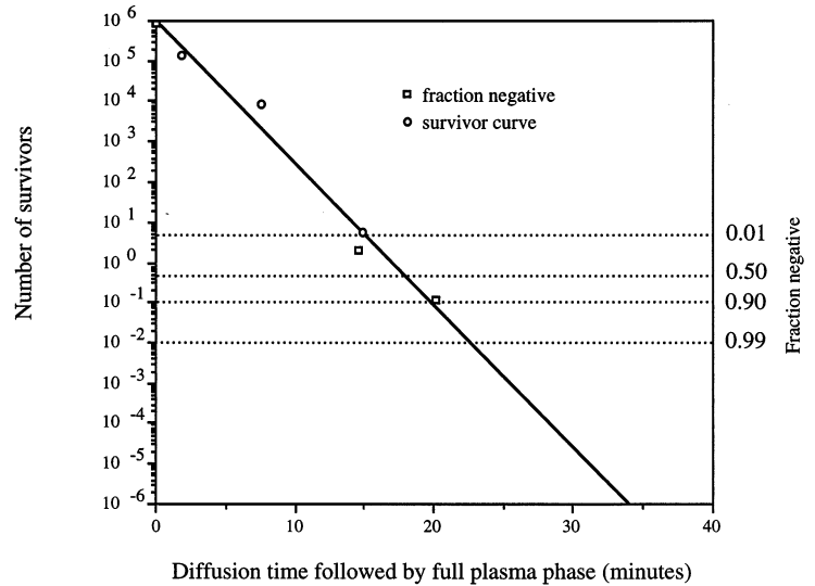
Figure 3. Amount of sterilization time required to achieve B. stearothermophilus spore levels of <10^{-6} using both survivor curve analysis and fraction negative analysis. The results yielded a similar linear regression relationship.
