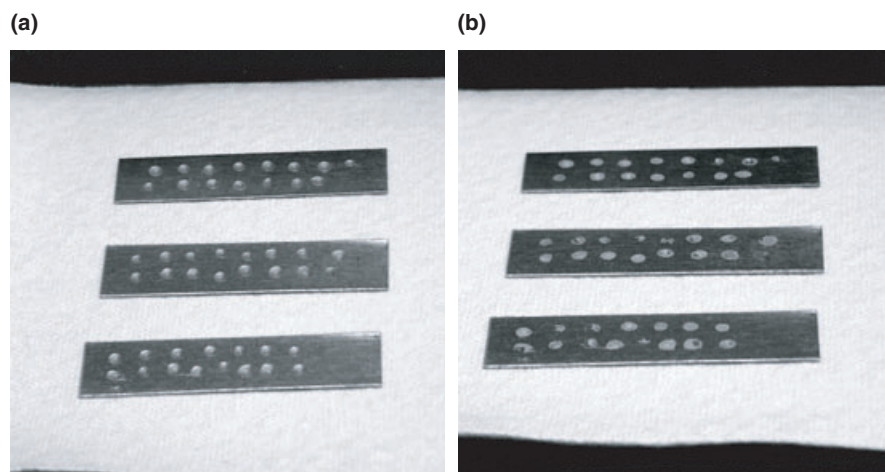
Fig. 1 Representative view of test coupons inoculated with 100 \mu\text{l} droplets containing approx. 1.0 \times 10^8 spores. (a) Image showing droplets immediately after application of spores. (b) Image of spores on test materials following overnight drying
